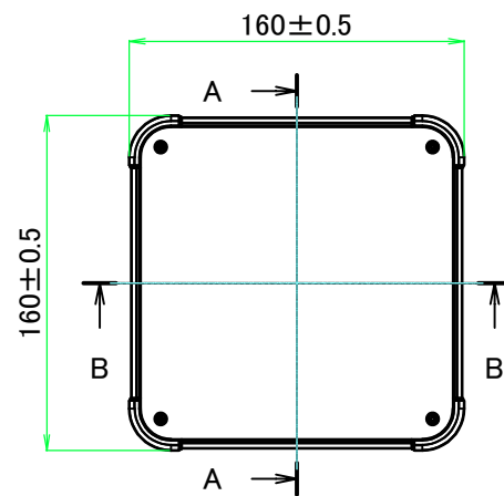
E view
