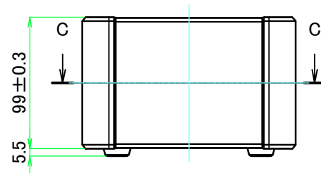
A view
